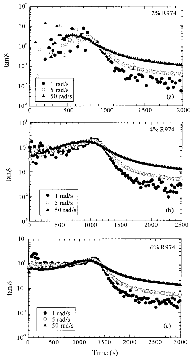
Figure 4. Loss tangent ( \tan \delta ) at various frequencies as a function of UV exposure time for the thiol-ene system containing various amounts of methyl-terminated (R974) colloidal fumed silica: (a) 2, (b) 4, and (c) 6 wt %.
