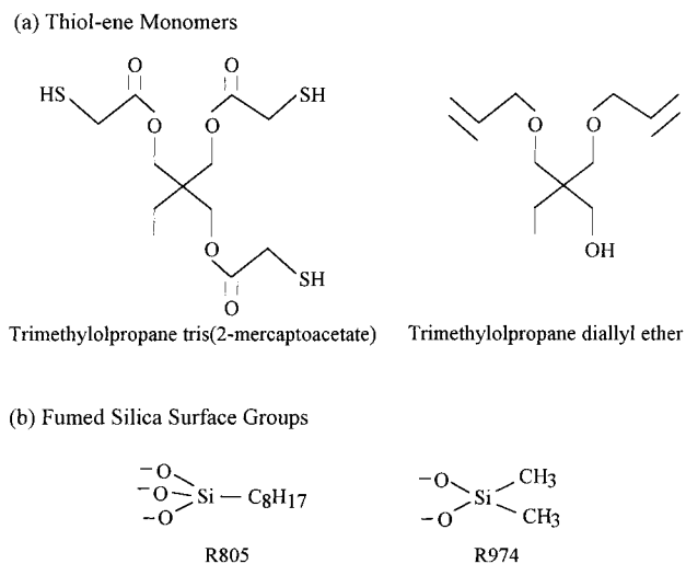
Figure 1. Schematic representation of the (a) chemical structures of the monomers comprising the UV cross-linkable system and (b) surface chemistries of the colloidal fumed silicas used. The R805 fumed silica contains octyl surface groups whereas the R974 fumed silica contains methyl-terminated groups.
