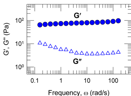
Figure 4. Foam rheology. Dynamic rheological data are shown for a foam prepared with hmC (5 mol % of C_{12} hydrophobes). The plot depicts the elastic modulus G' (filled circles) and the viscous modulus G'' (unfilled triangles) as functions of frequency. The foam shows an elastic (solid-like) response.
