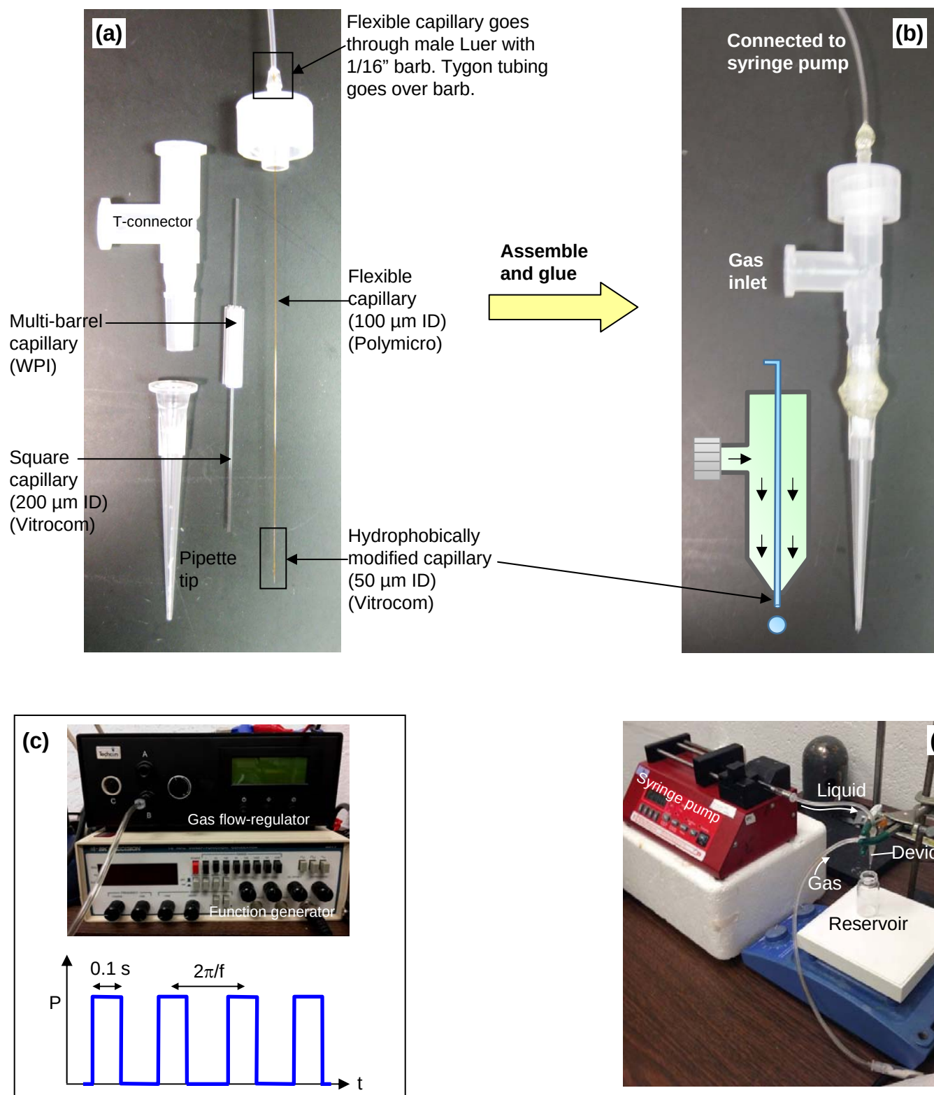
Figure S1. Photos and details of the microfluidic setup used to generate capsules and MCCs. The components of the microfluidic device are shown in (a). After assembly and gluing with epoxy, the final device is shown in (b). The schematic in Figure 2 is reproduced as an inset to show the correspondence to the actual device. Note that the liquid finally emerges out of the capillary with a 50 \mu\text{m} ID. In (c), a photo of the function generator and gas flow-regulator is shown. The gas is sent as pulses at a pressure P , with each pulse over a duration of 0.1 s and with the spacing between pulses dictated by the frequency f . In (d), a photo of the device in operation is shown, along with the syringe pump and collection reservoir (vial).
