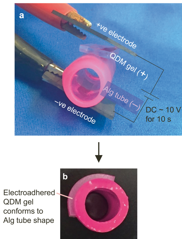
Fig. 2 Electroadhesion of QDM gel-strip to Alg tube. a The gel and tube are contacted with graphite electrodes, with the positive electrode touching the cationic QDM gel and the negative electrode touching the anionic Alg tube. b Upon applying 10 V of DC for 10 s, the gel gets tightly adhered to the tube and conforms to the tube shape. In cases where a puncture is made in the tube wall, adhesion of the gel over the puncture location serves to patch up the puncture (see next figure).
