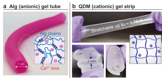
Fig. 1 Gels used in our electroadhesion studies. a Anionic gel of alginate (Alg), crosslinked by divalent \text{Ca}^{2+} cations. The gel is made in the form of a hollow tube. b Cationic QDM gel strip, made by polymerization of acrylamide derivatives. The photos show that the gel is elastic, stretchable and flexible. Schematics of the gel structure are shown as insets in each case.
